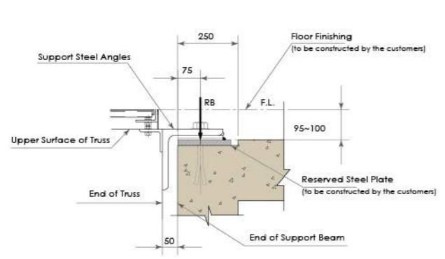
End Support Drawing
