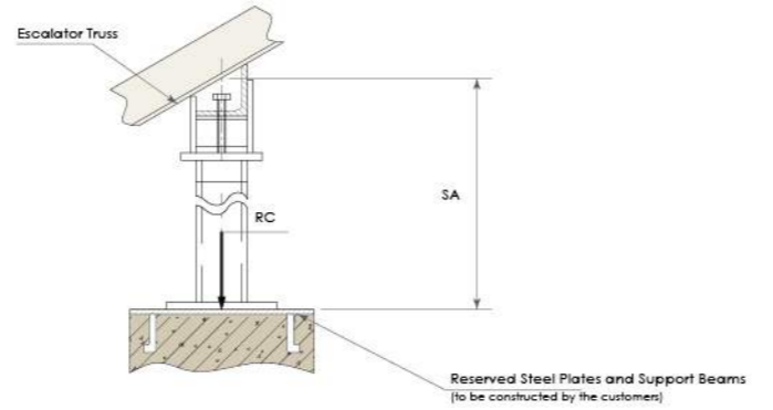
Intermediate Support Drawing
