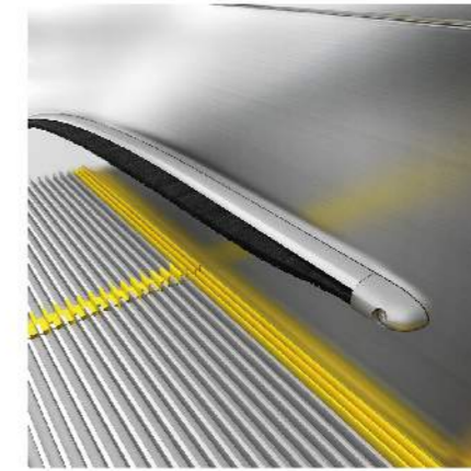
Brush - Pinch-Proof Device at the Skirting
